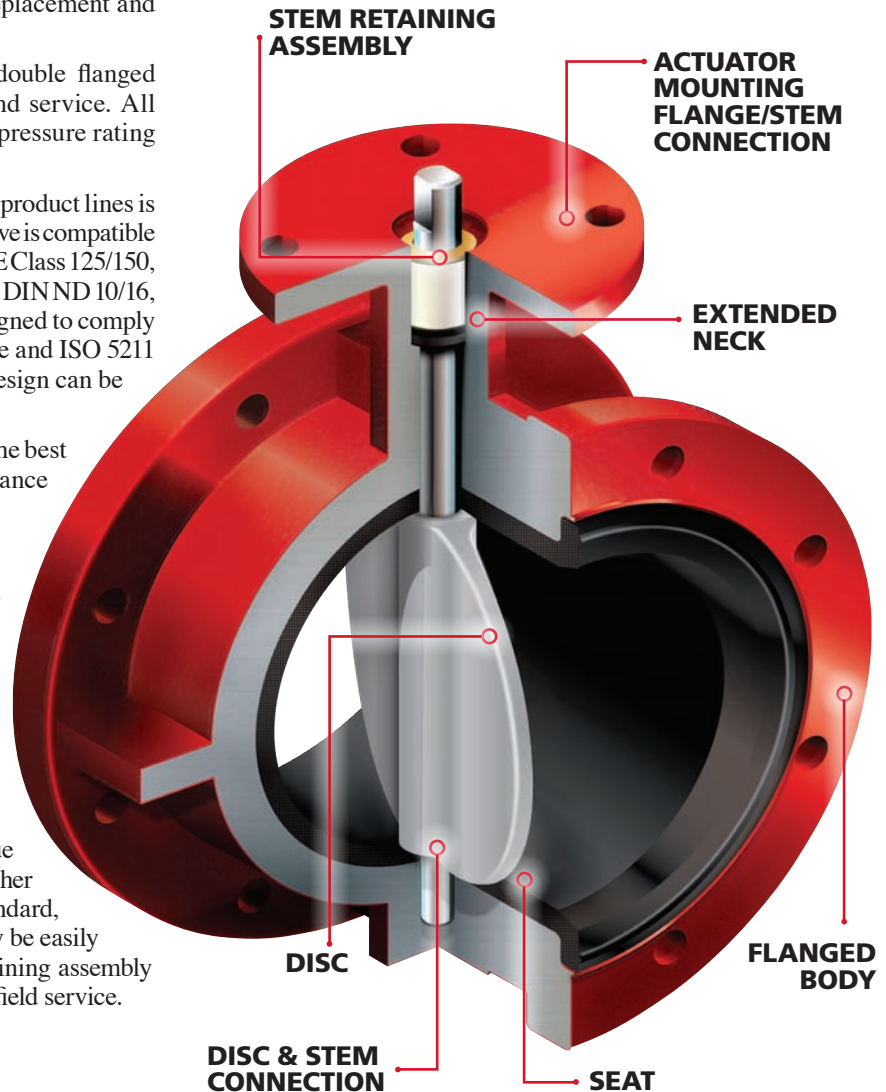
STEM RETAINING ASSEMBLY STEM BUSHING STEM SEAL
