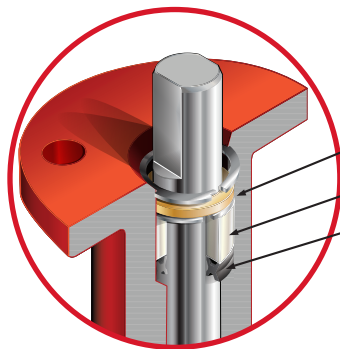
STEM RETAINING ASSEMBLY STEM BUSHING STEM SEAL
