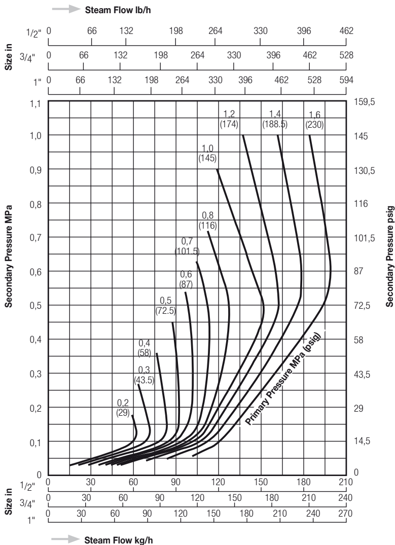
Capacity Chart REC1
