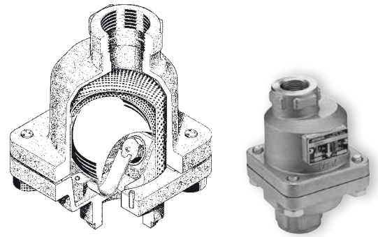
Vertical installation
