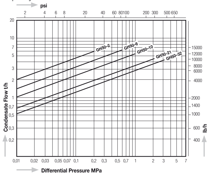
Capacity Chart GH50
