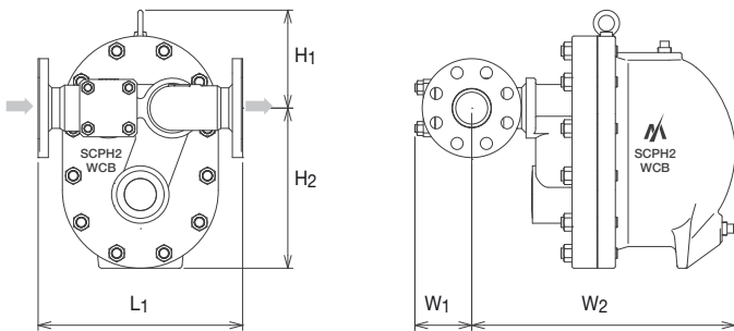
Dimensions GH60
