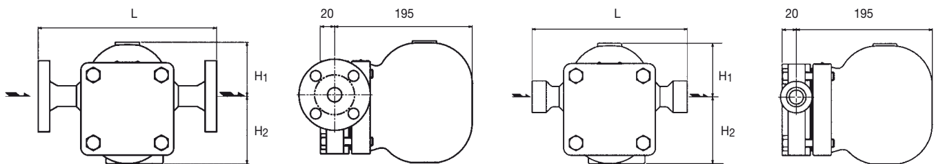
GTH12-F Flanged
